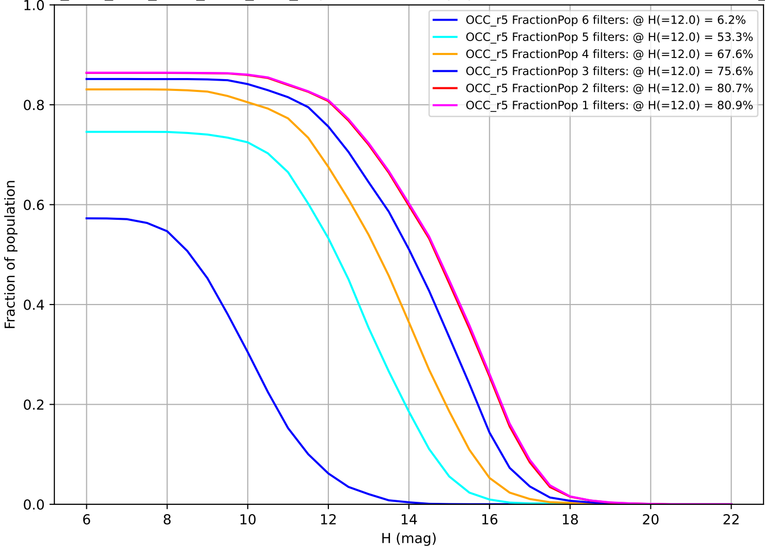
ddf_acor_sf10_lsf30_lsr20_v3.4_10yrs: Fraction of population with colors in X filters OCC_r5
