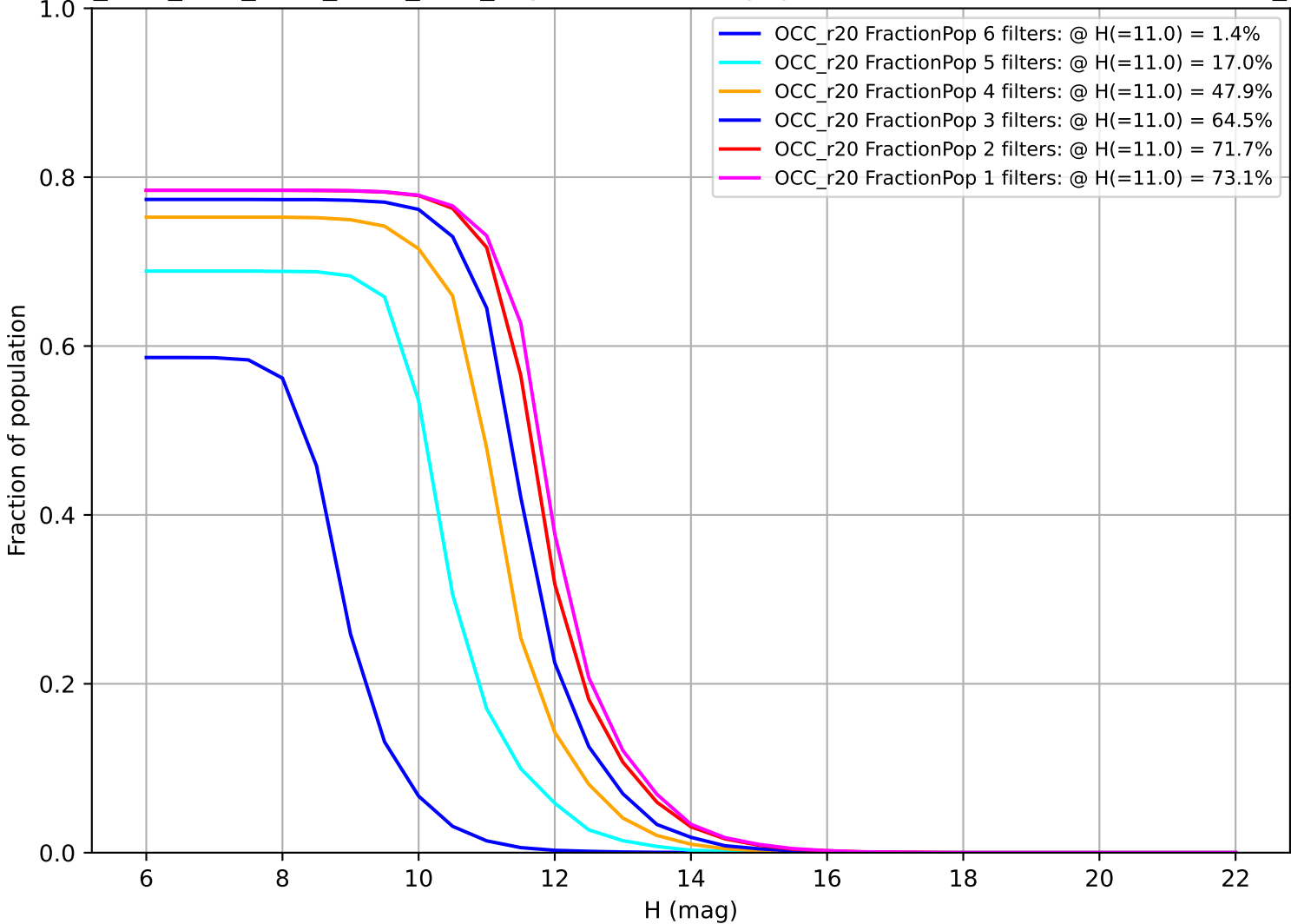
ddf_acor_sf10_lsf30_lsr20_v3.4_10yrs: Fraction of population with colors in X filters OCC_r20
