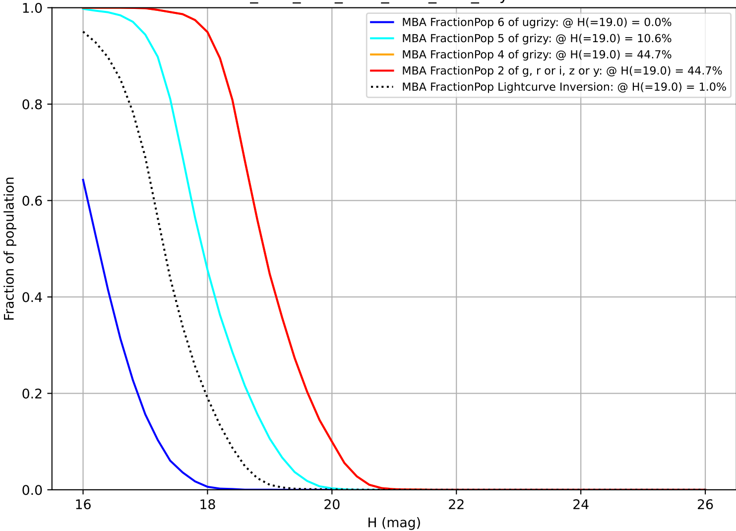
ddf_acor_sf10_lsf30_lsr20_v3.4_10yrs MBA
