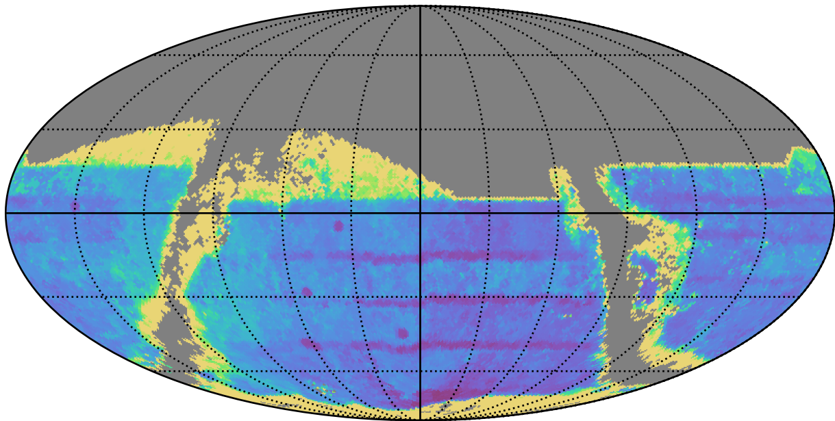
ddf_acor_sf10_lsf30_lsr20_v3.4_10yrs : TDC_accuracy
