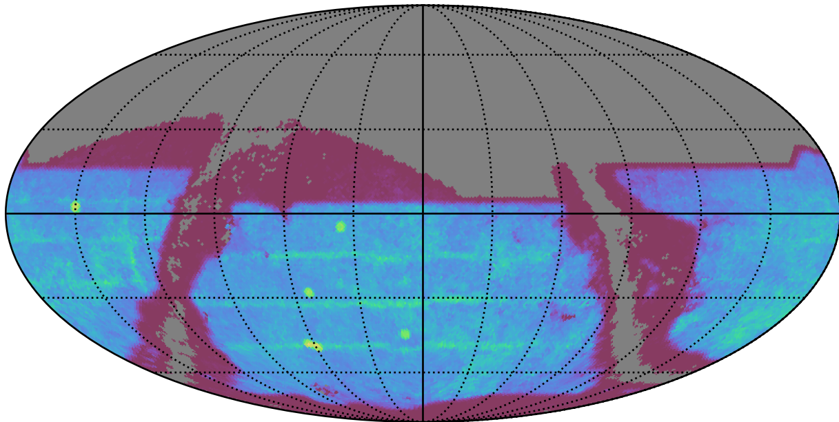
ddf_acor_sf10_lsf30_lsr20_v3.4_10yrs : SNSLMetric
