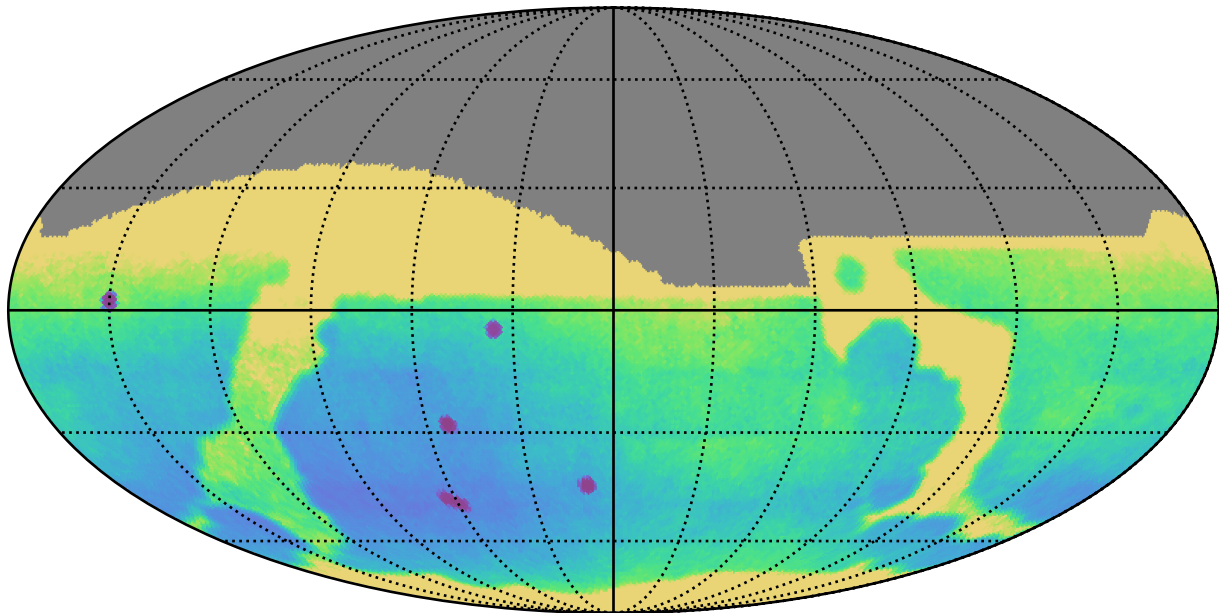
ddf_acor_sf10_lsf30_lsr20_v3.4_10yrs : Parallax Uncert @ 24.0
