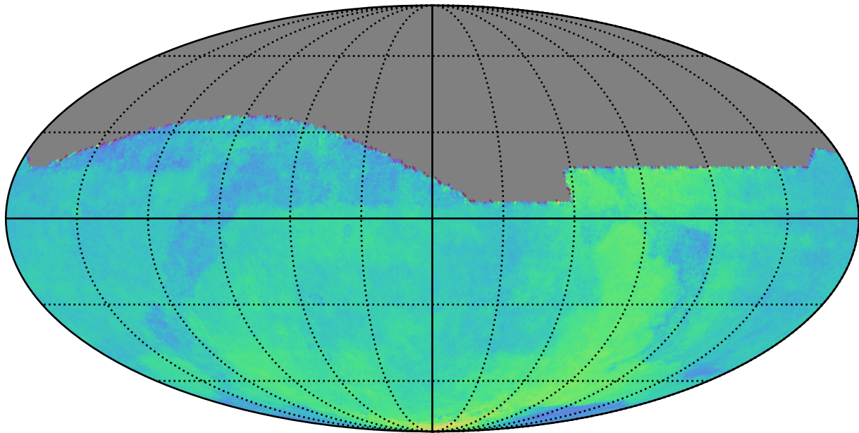
ddf_acor_sf10_lsf30_lsr20_v3.4_10yrs : Parallax Coverage @ 22.4
