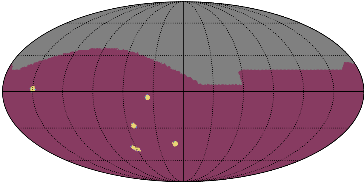
ddf_acor_sf10_lsf30_lsr20_v3.4_10yrs : NumberOfQuickRevisits
