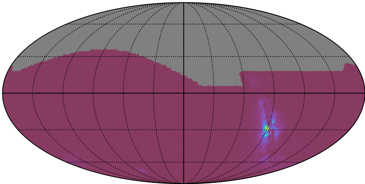
ddf_acor_sf10_lsf30_lsr20_v3.4_10yrs : NlcPoints
