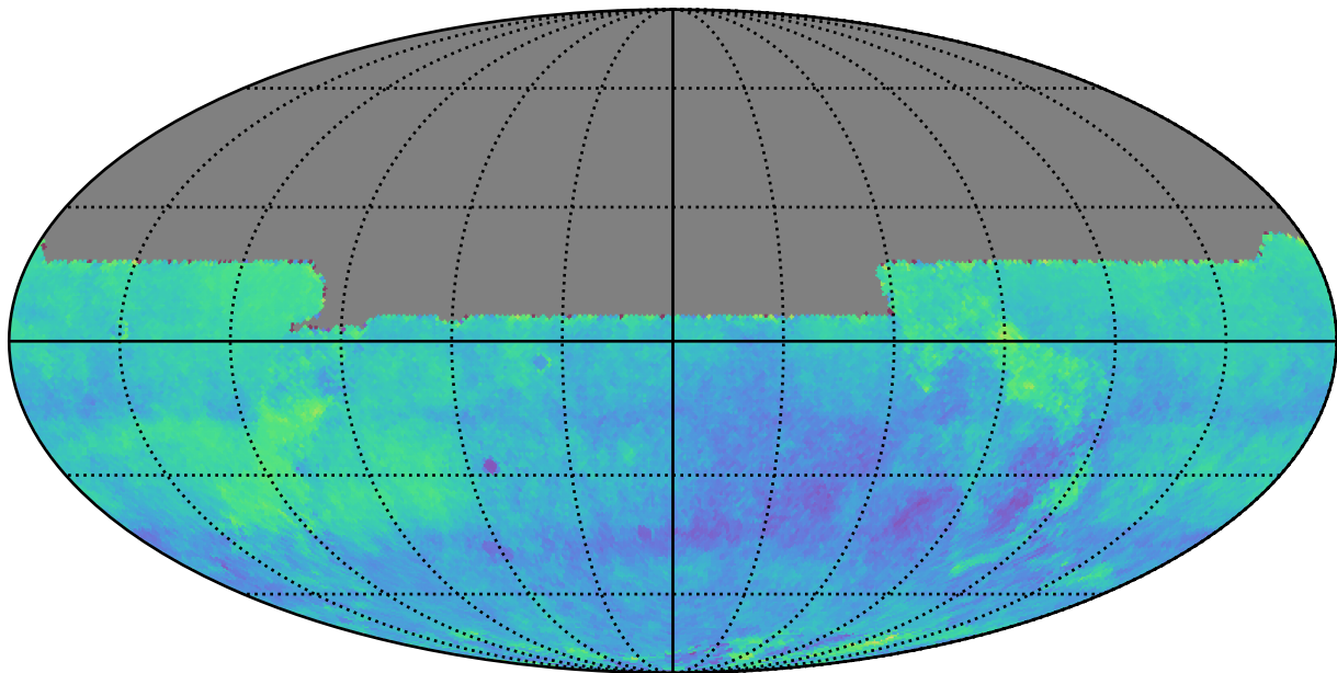
ddf_acor_sf10_lsf30_lsr20_v3.4_10yrs y: Kuiper rotSkyPos
