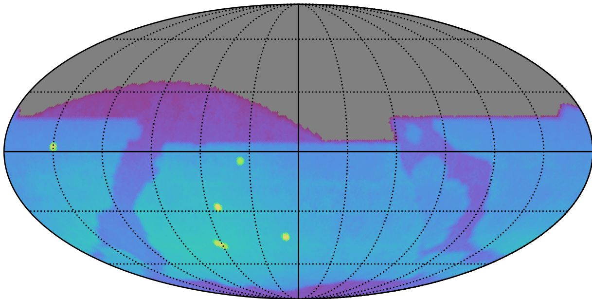
ddf_acor_sf10_lsf30_lsr20_v3.4_10yrs : Brown Dwarf, L7
