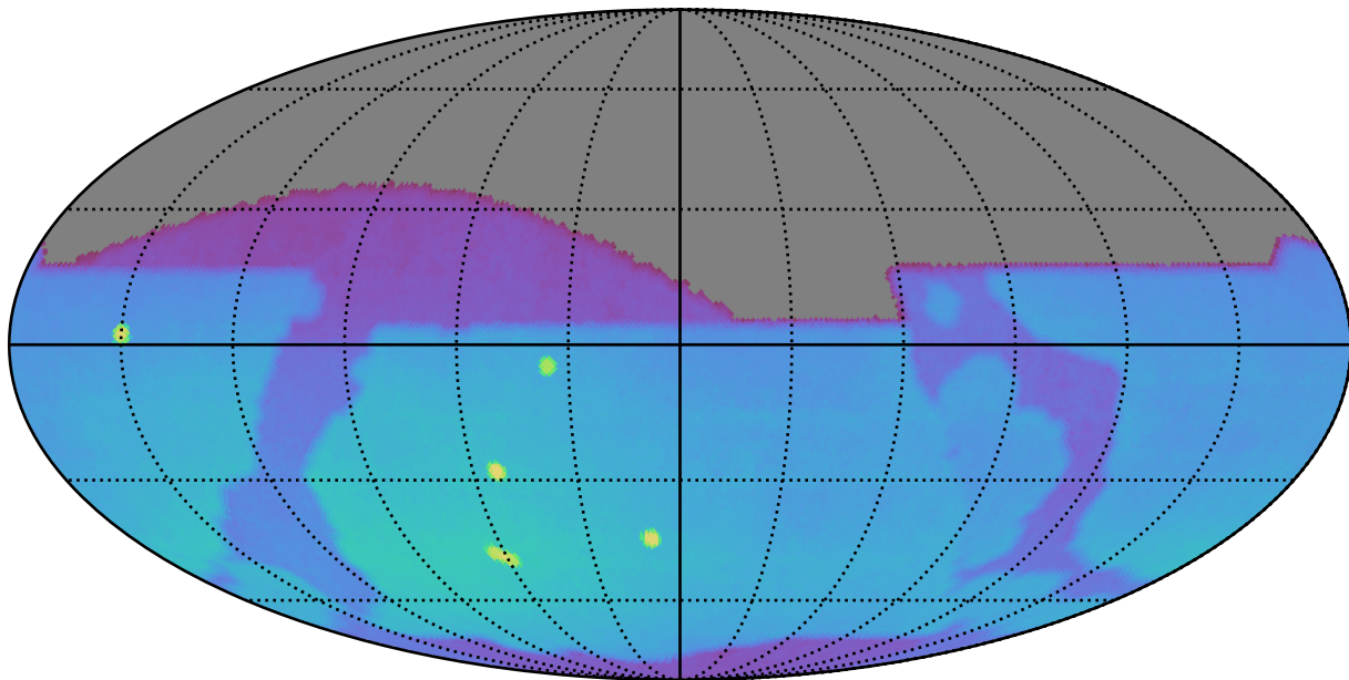
ddf_acor_sf10_lsf30_lsr20_v3.4_10yrs : Brown Dwarf, L4
