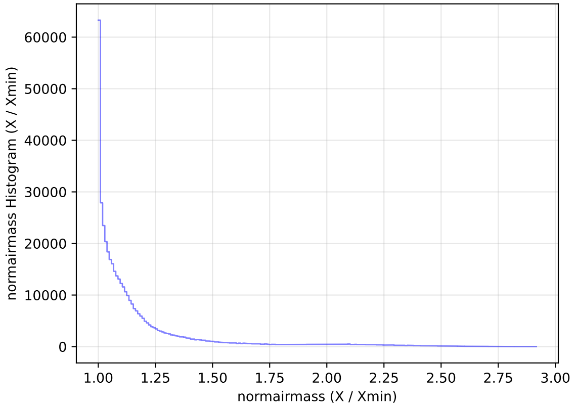
ddf_acor_sf10_lsf30_lsr20_v3.4_10yrs All sky z band: normairmass Histogram
