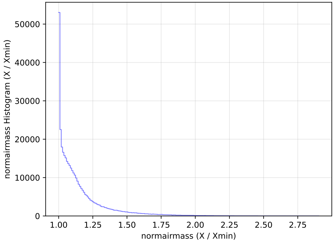
ddf_acor_sf10_lsf30_lsr20_v3.4_10yrs All sky y band: normairmass Histogram
