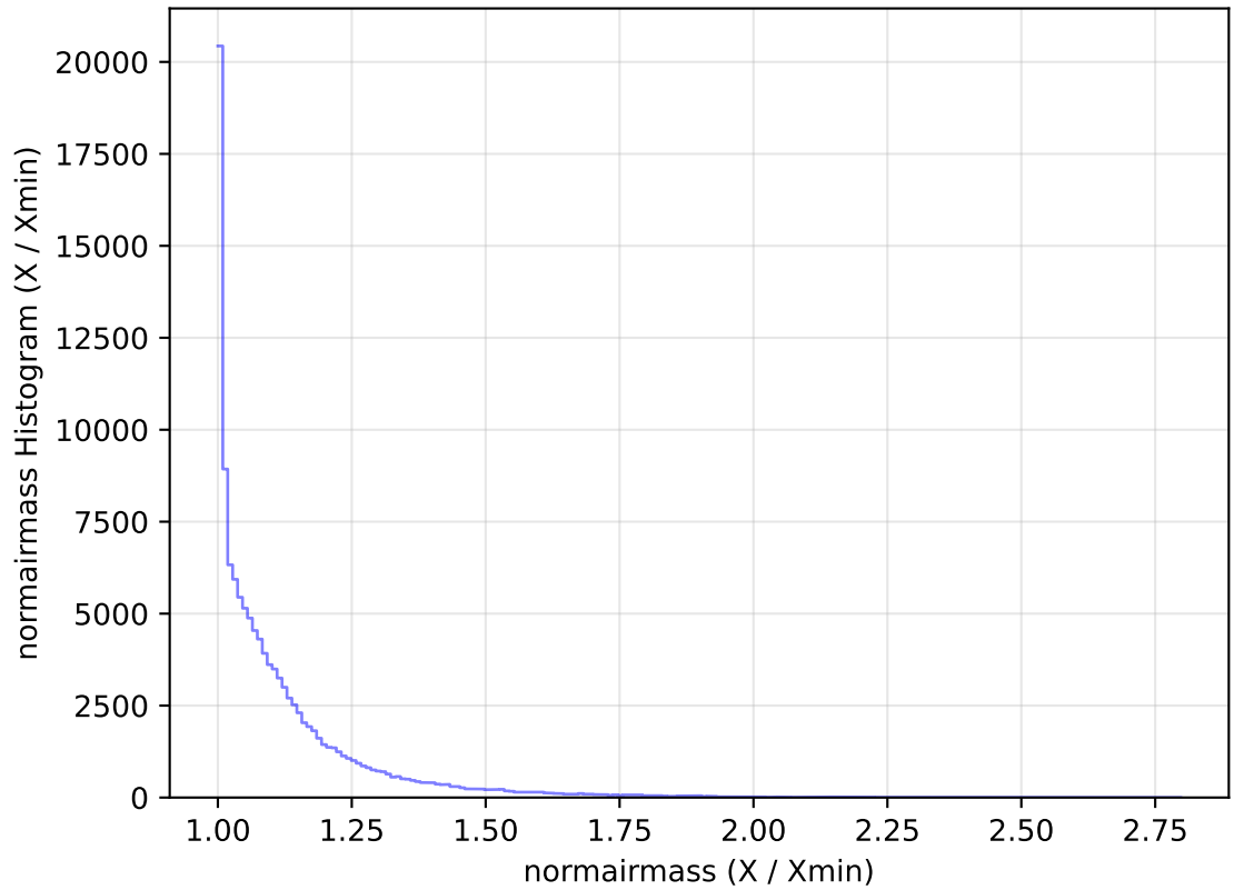
ddf_acor_sf10_lsf30_lsr20_v3.4_10yrs All sky u band: normairmass Histogram
