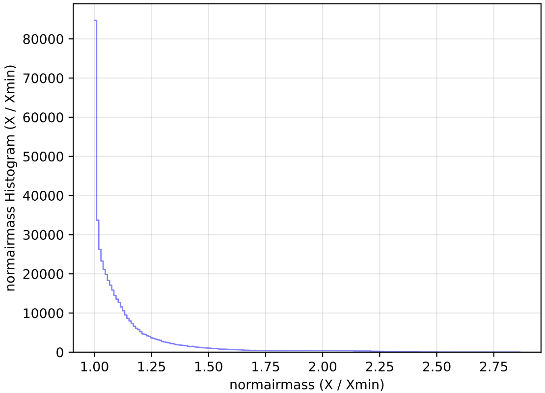
ddf_acor_sf10_lsf30_lsr20_v3.4_10yrs All sky r band: normairmass Histogram
