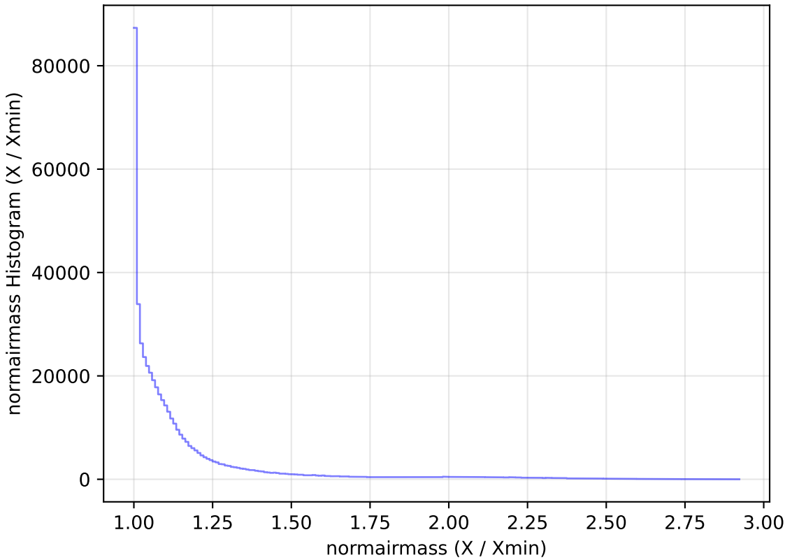
ddf_acor_sf10_lsf30_lsr20_v3.4_10yrs All sky i band: normairmass Histogram
