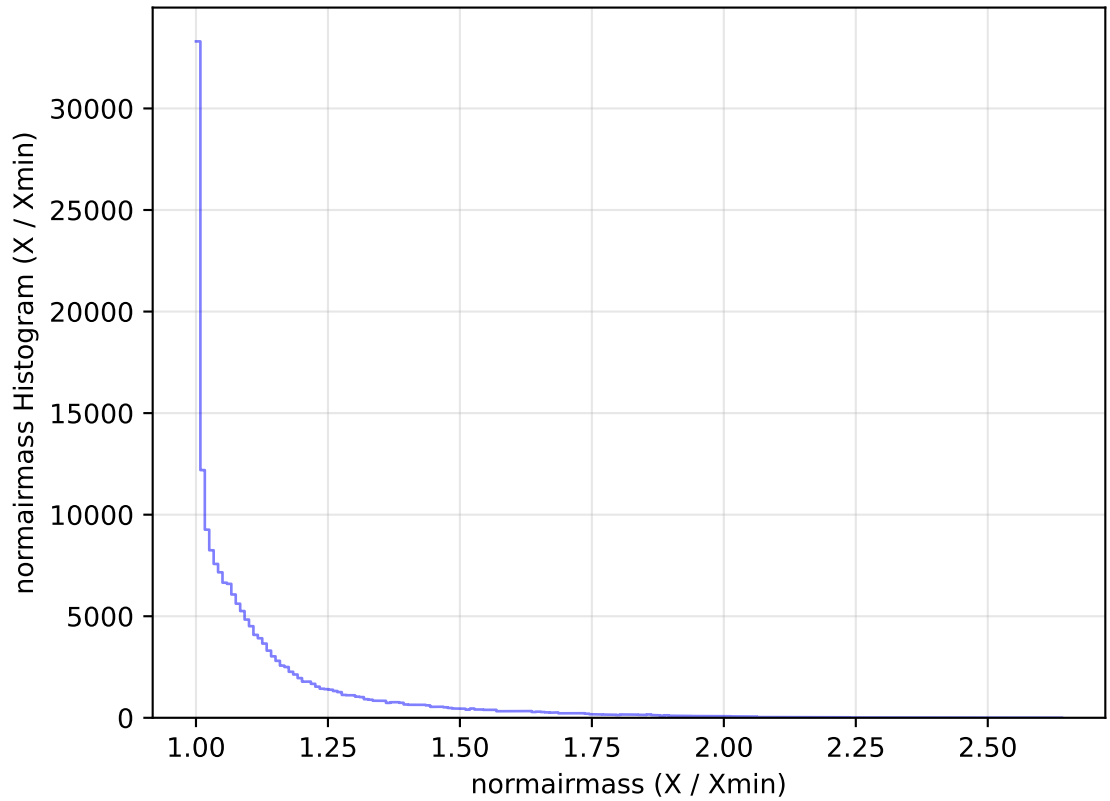
ddf_acor_sf10_lsf30_lsr20_v3.4_10yrs All sky g band: normairmass Histogram
