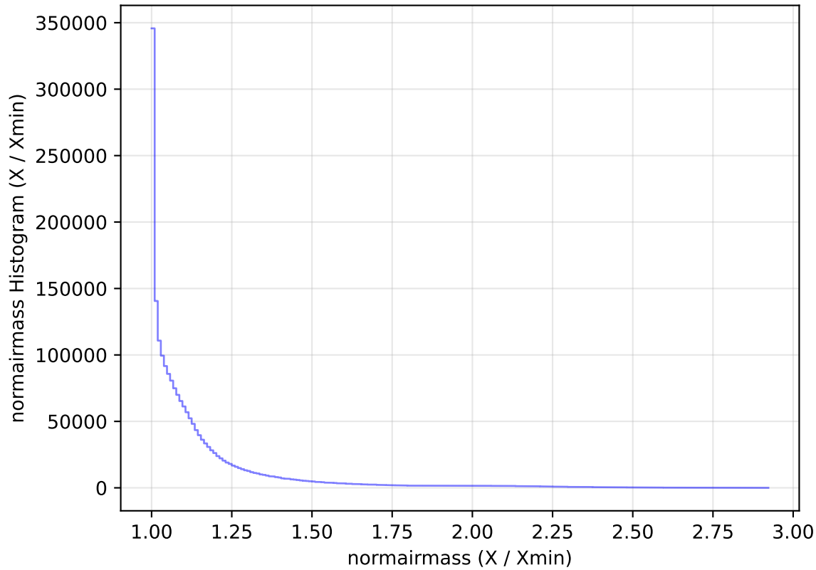
ddf_acor_sf10_lsf30_lsr20_v3.4_10yrs All sky all bands: normairmass Histogram
