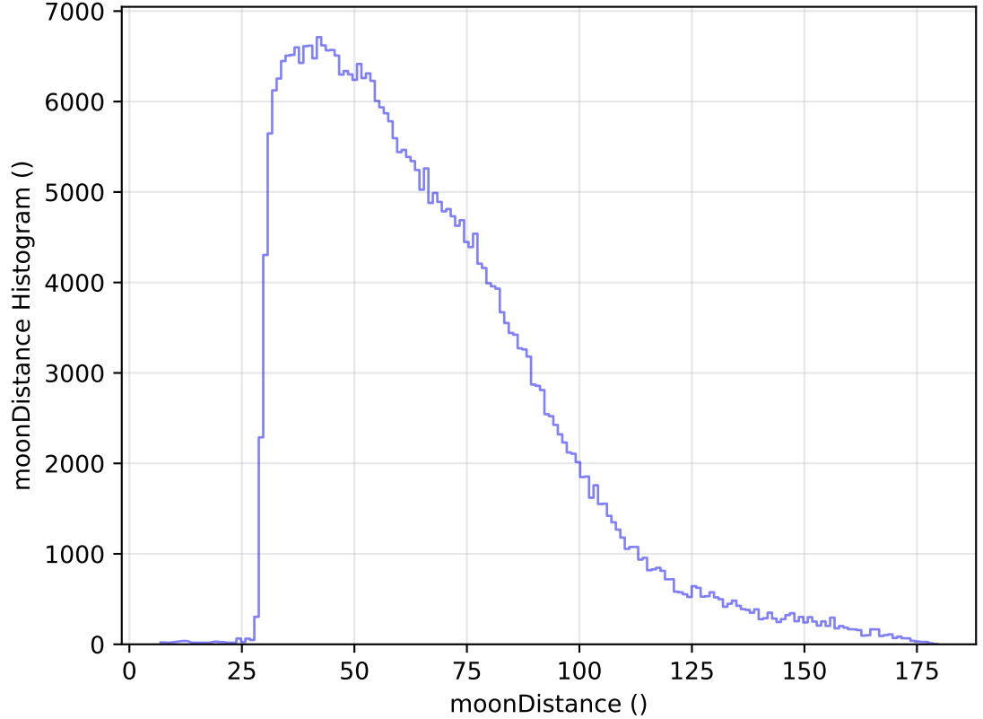
ddf_acor_sf10_lsf30_lsr20_v3.4_10yrs WFD y band: moonDistance Histogram
