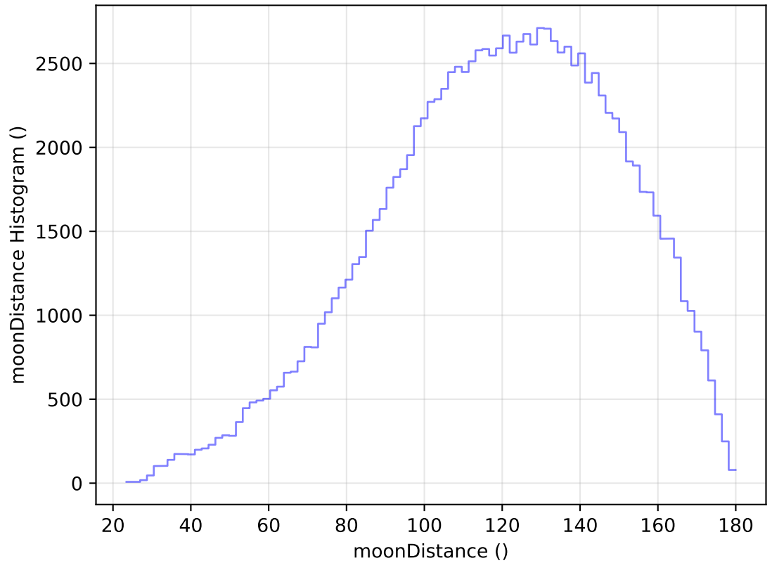
ddf_acor_sf10_lsf30_lsr20_v3.4_10yrs WFD u band: moonDistance Histogram
