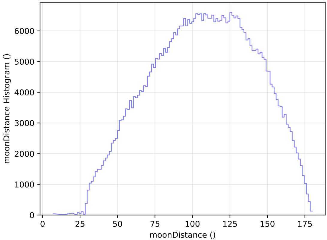
ddf_acor_sf10_lsf30_lsr20_v3.4_10yrs WFD r band: moonDistance Histogram
