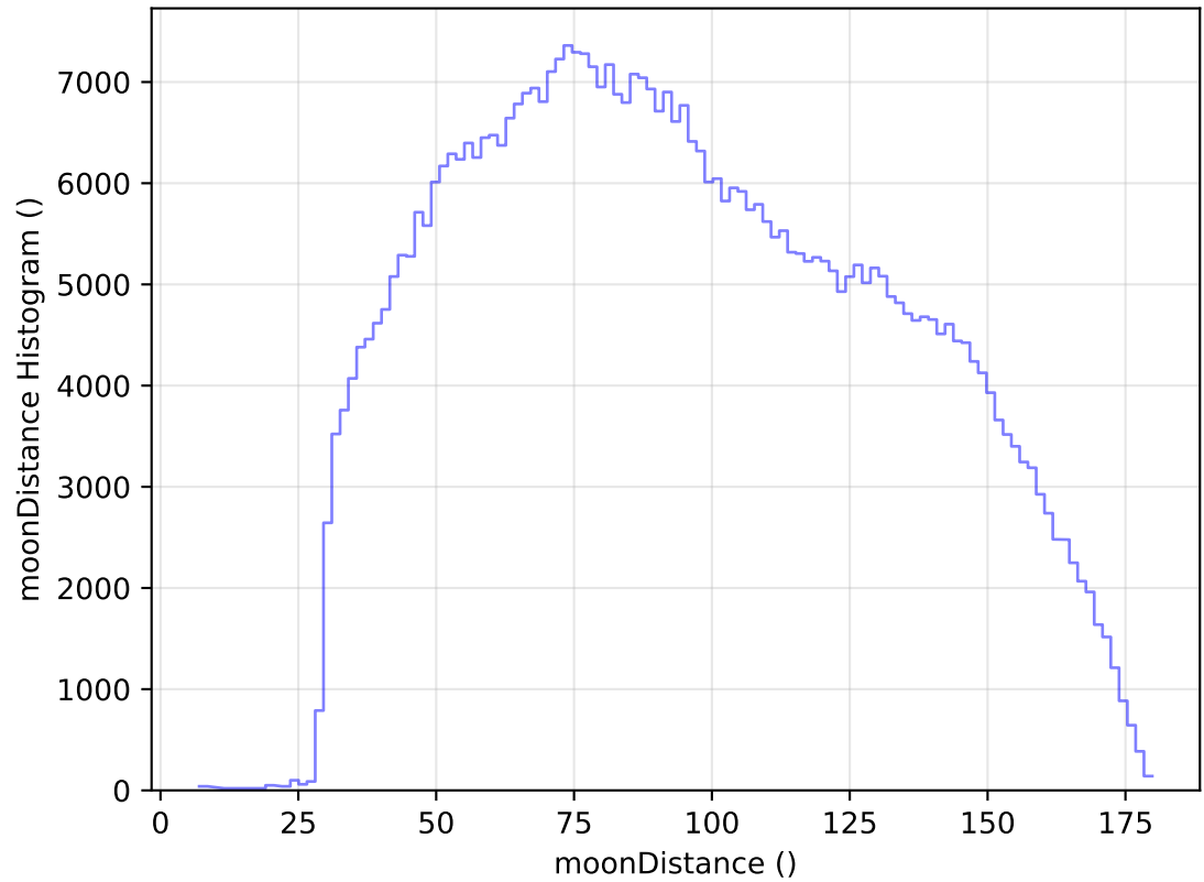
ddf_acor_sf10_lsf30_lsr20_v3.4_10yrs WFD i band: moonDistance Histogram
