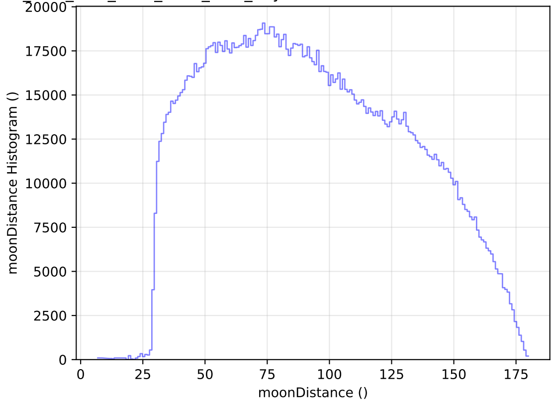
ddf_acor_sf10_lsf30_lsr20_v3.4_10yrs WFD all bands: moonDistance Histogram
