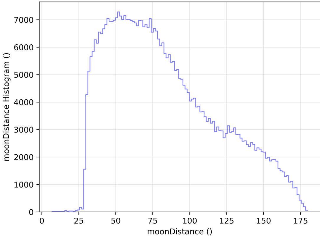
ddf_acor_sf10_lsf30_lsr20_v3.4_10yrs All sky z band: moonDistance Histogram
