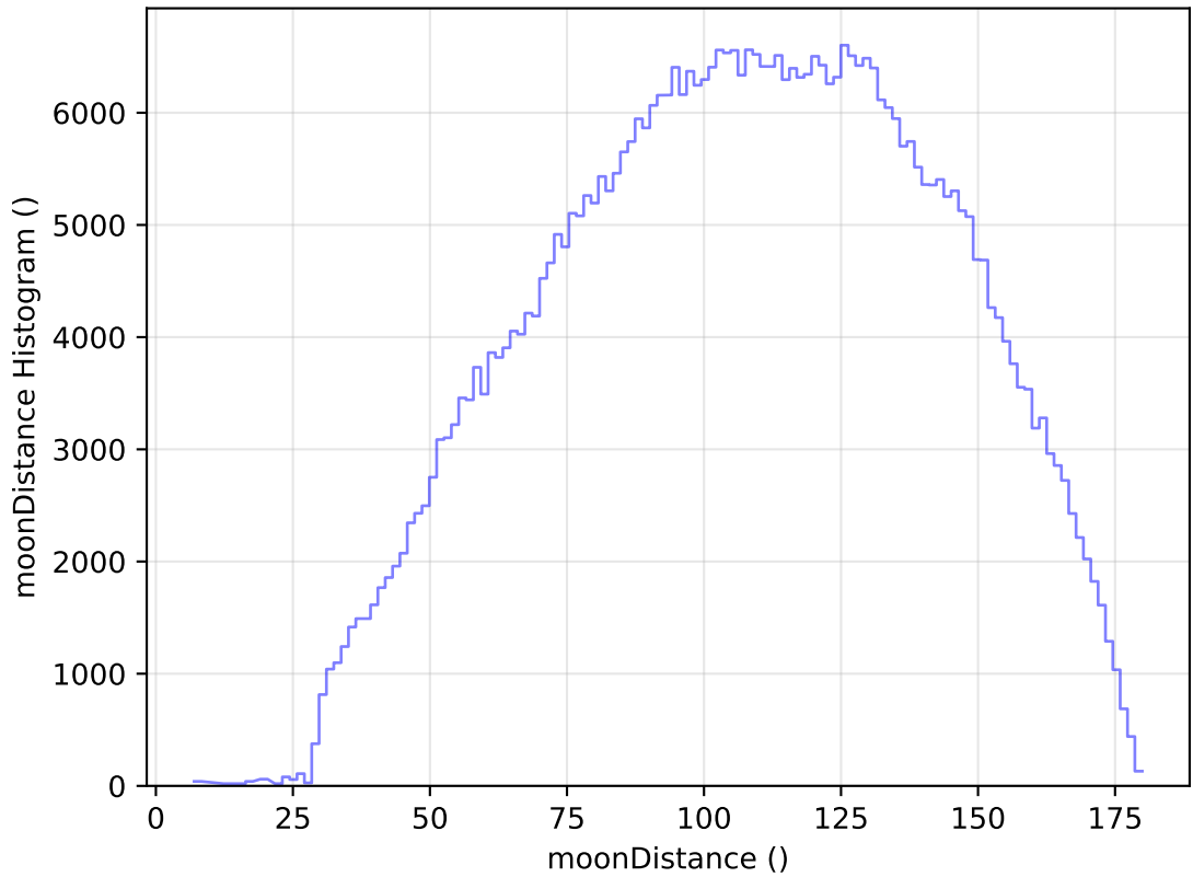
ddf_acor_sf10_lsf30_lsr20_v3.4_10yrs All sky r band: moonDistance Histogram
