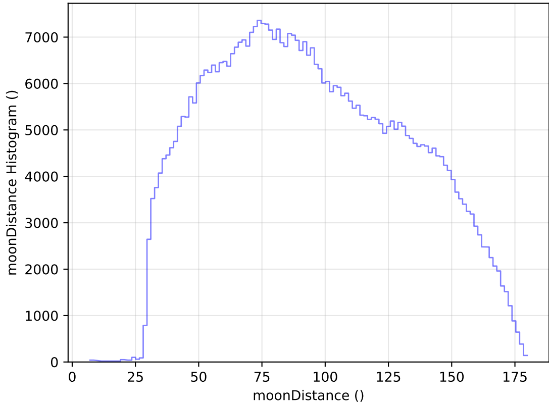
ddf_acor_sf10_lsf30_lsr20_v3.4_10yrs All sky i band: moonDistance Histogram
