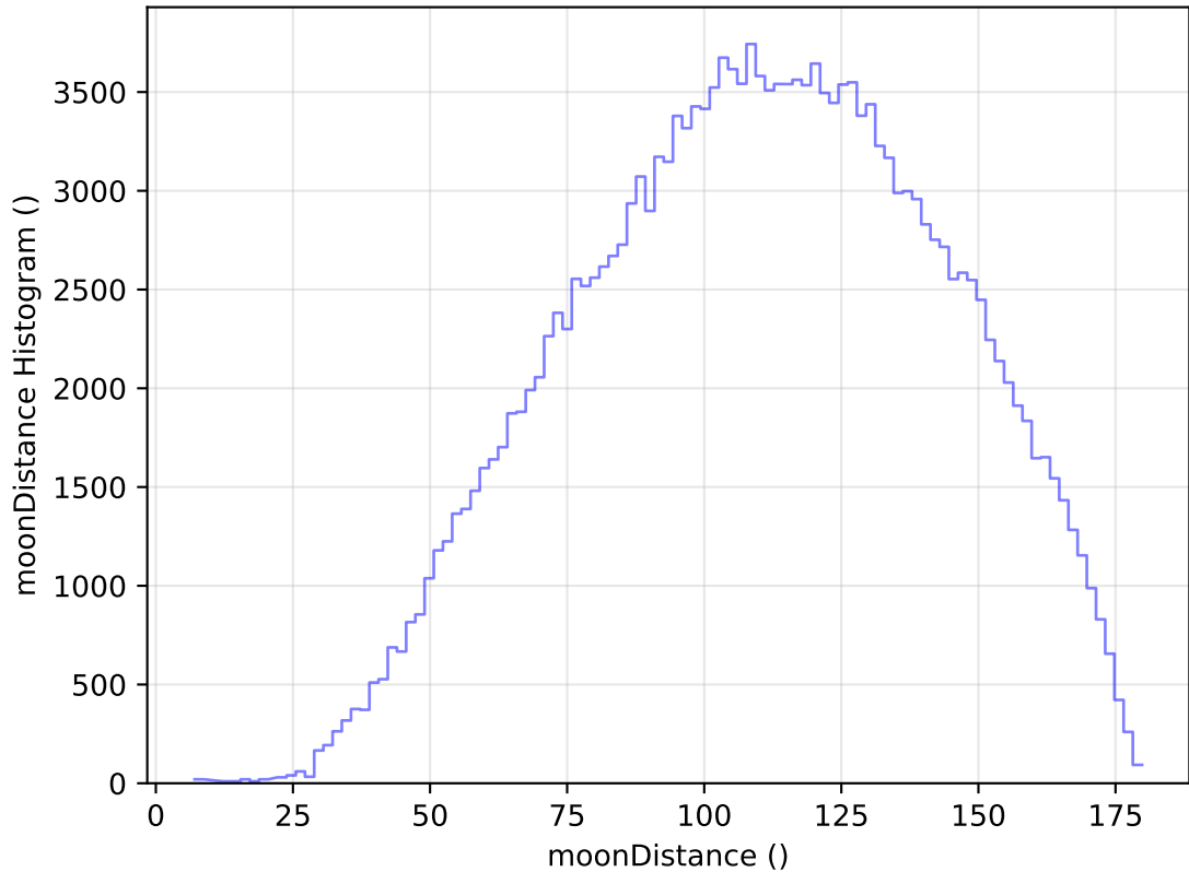
ddf_acor_sf10_lsf30_lsr20_v3.4_10yrs All sky g band: moonDistance Histogram
