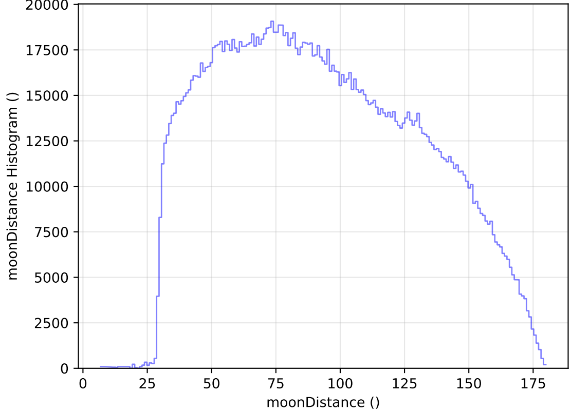
ddf_acor_sf10_lsf30_lsr20_v3.4_10yrs All sky all bands: moonDistance Histogram
