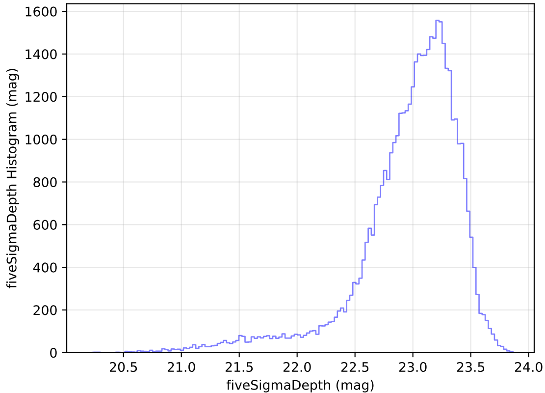
ddf_acor_sf10_lsf30_lsr20_v3.4_10yrs Yr 1 z band: fiveSigmaDepth Histogram
