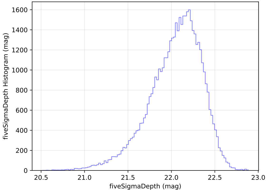
ddf_acor_sf10_lsf30_lsr20_v3.4_10yrs Yr 1 y band: fiveSigmaDepth Histogram
