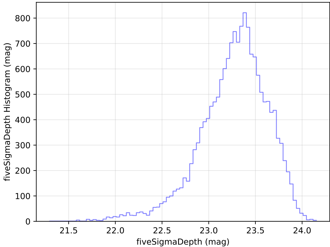
ddf_acor_sf10_lsf30_lsr20_v3.4_10yrs Yr 1 u band: fiveSigmaDepth Histogram
