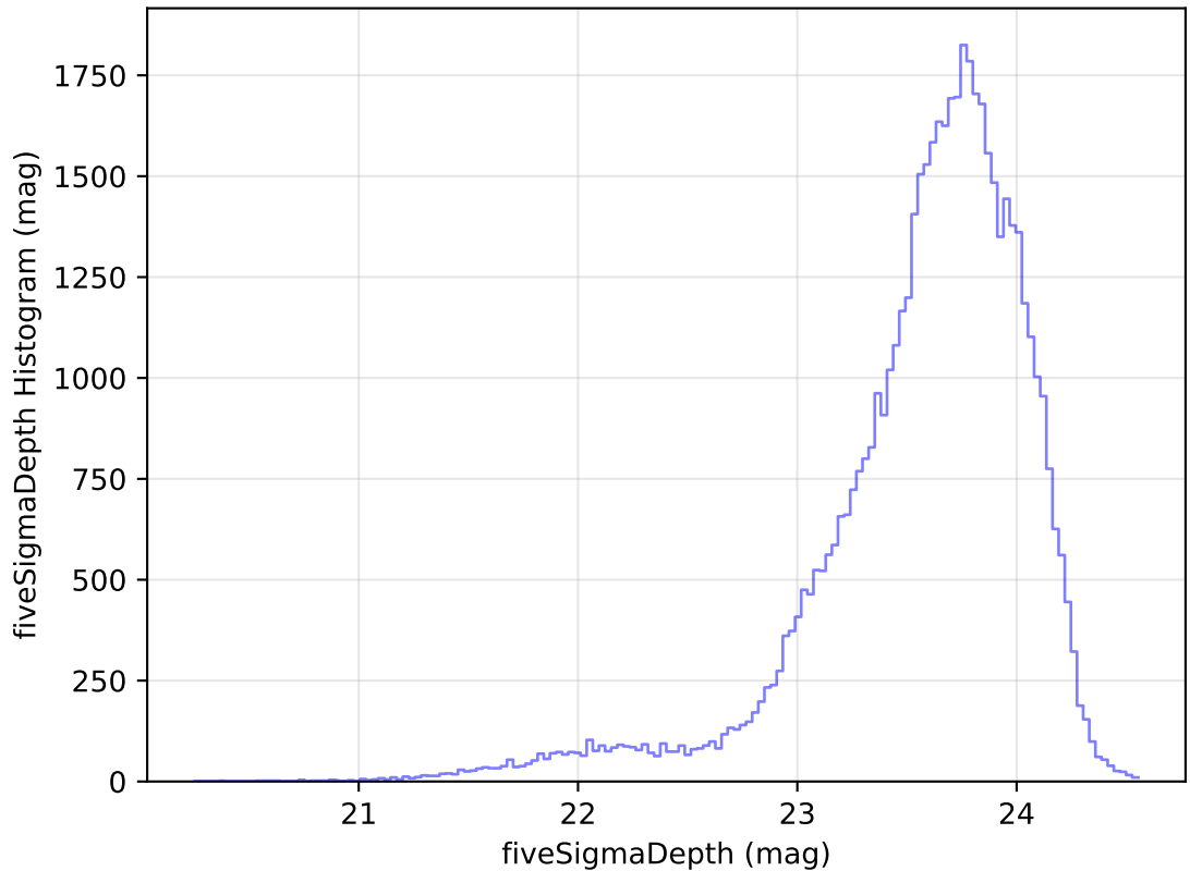
ddf_acor_sf10_lsf30_lsr20_v3.4_10yrs Yr 1 i band: fiveSigmaDepth Histogram
