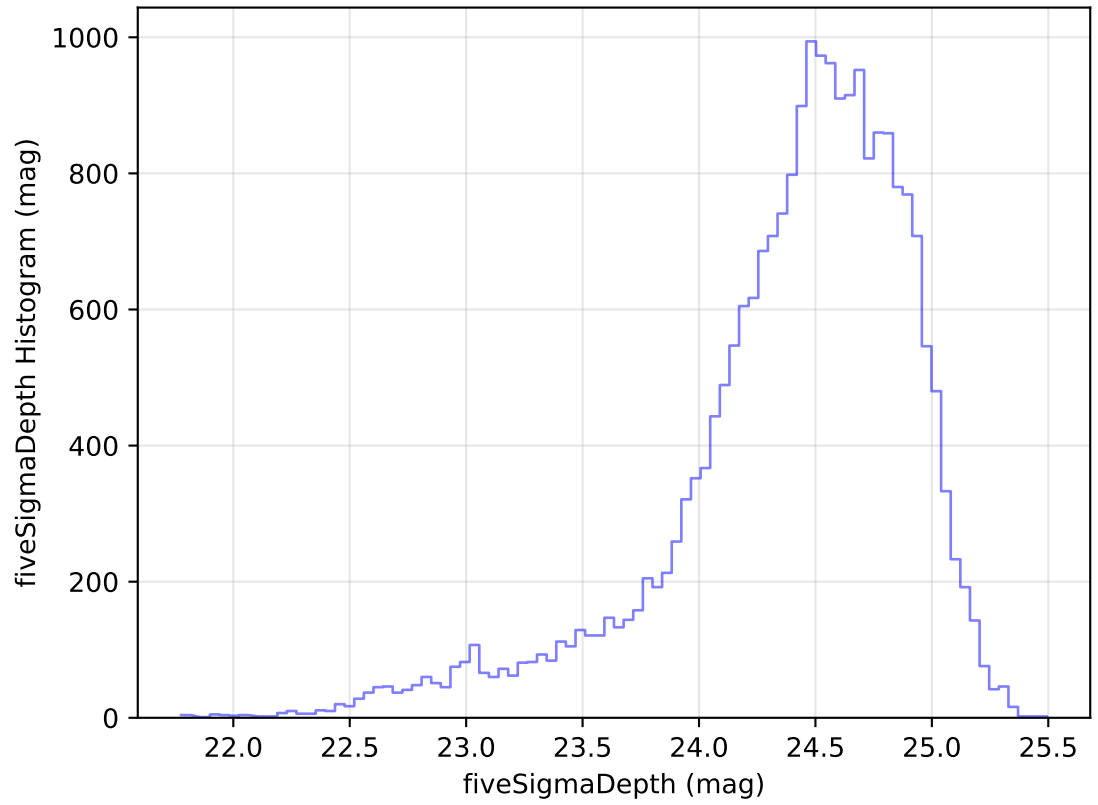
ddf_acor_sf10_lsf30_lsr20_v3.4_10yrs Yr 1 g band: fiveSigmaDepth Histogram
