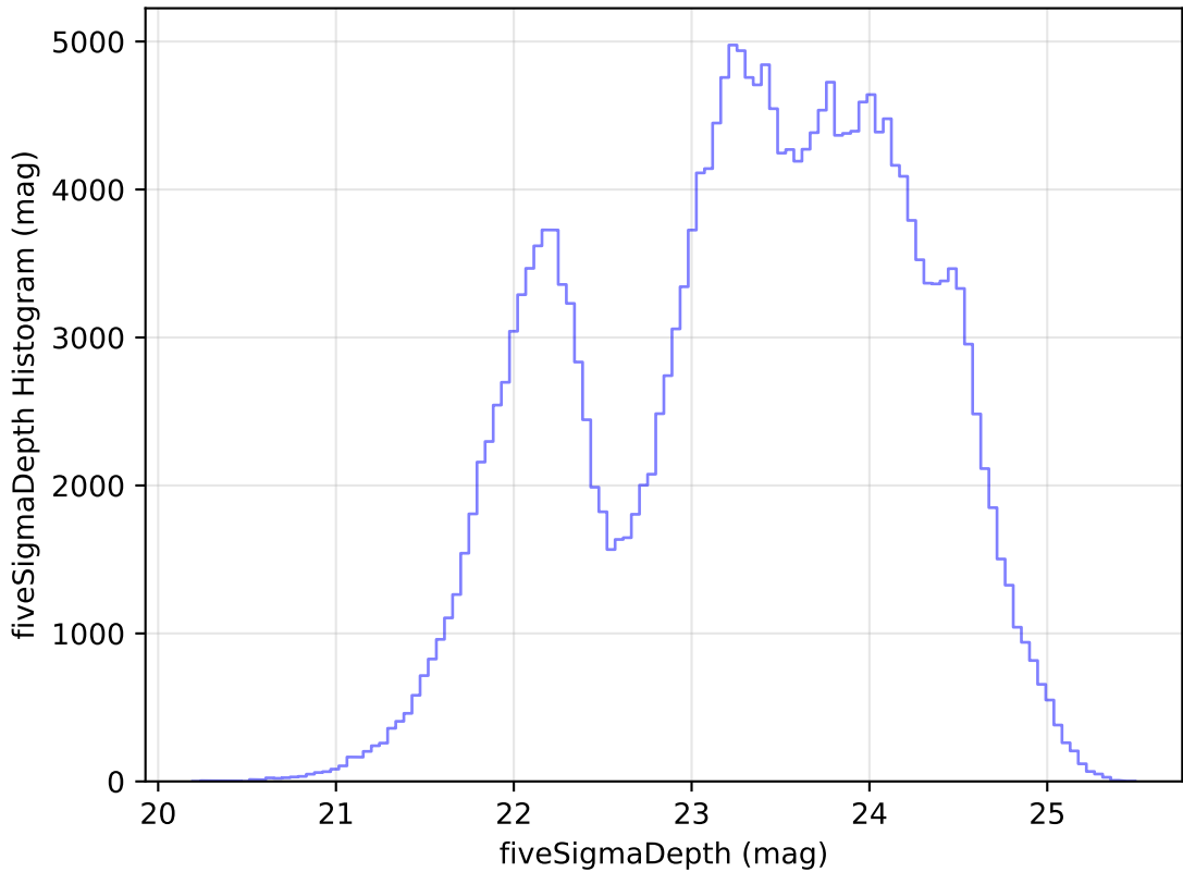
ddf_acor_sf10_lsf30_lsr20_v3.4_10yrs Yr 1 all bands: fiveSigmaDepth Histogram
