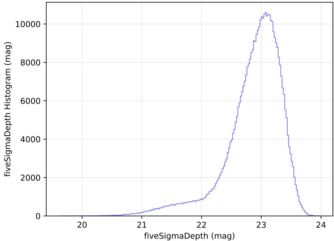
ddf_acor_sf10_lsf30_lsr20_v3.4_10yrs WFD z band: fiveSigmaDepth Histogram
