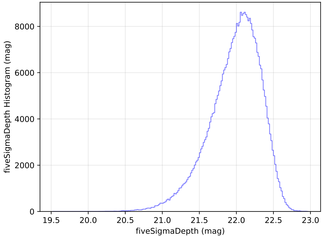
ddf_acor_sf10_lsf30_lsr20_v3.4_10yrs WFD y band: fiveSigmaDepth Histogram
