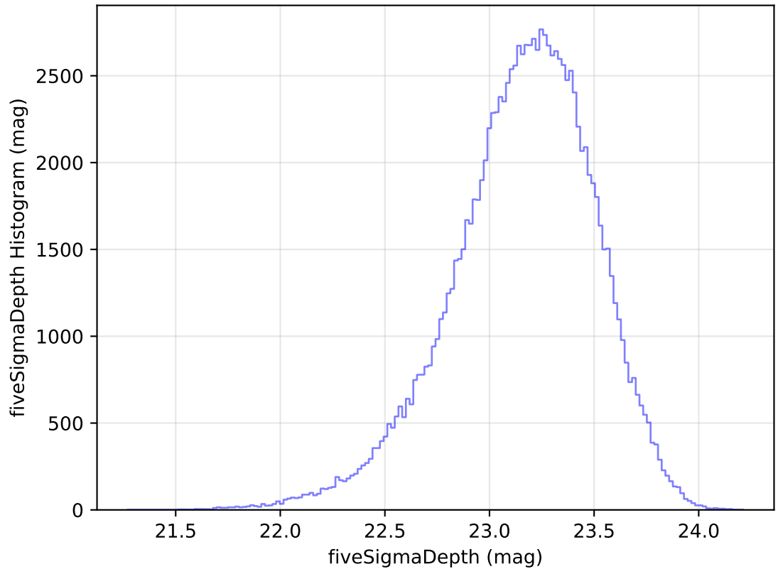
ddf_acor_sf10_lsf30_lsr20_v3.4_10yrs WFD u band: fiveSigmaDepth Histogram
