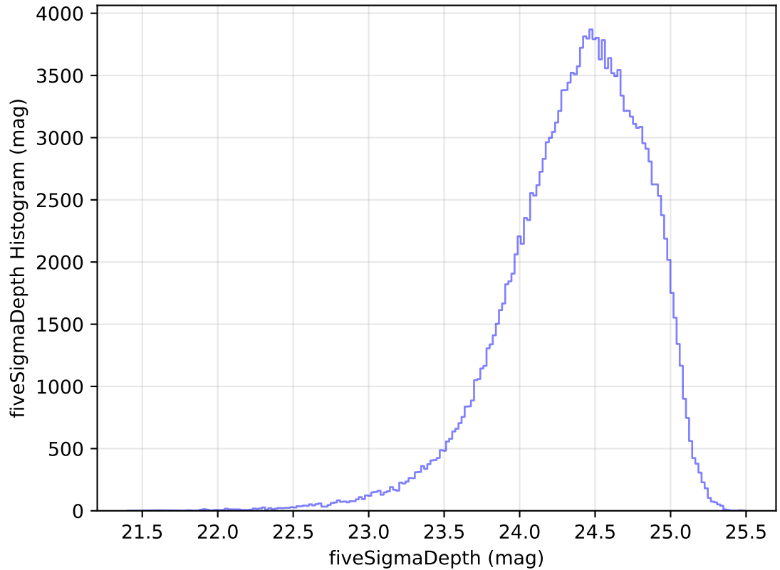
ddf_acor_sf10_lsf30_lsr20_v3.4_10yrs WFD g band: fiveSigmaDepth Histogram
