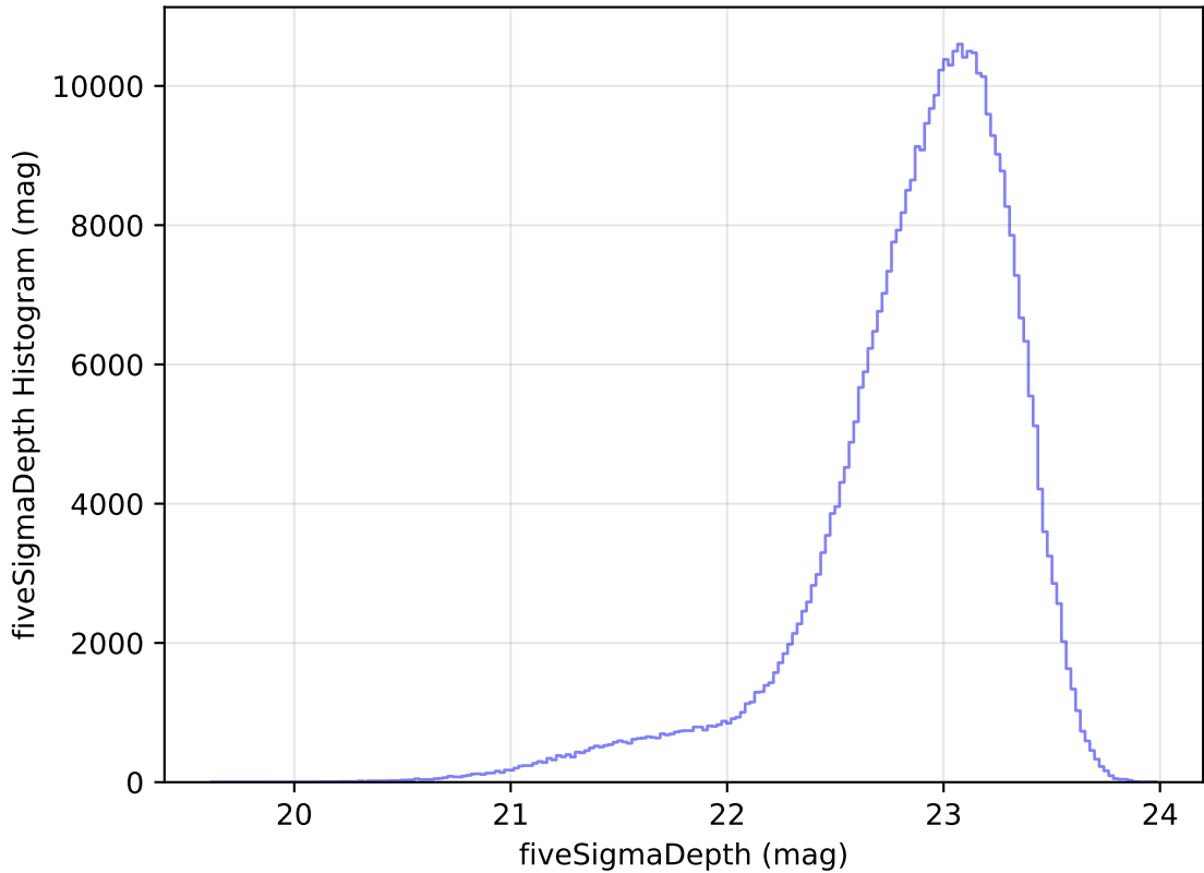
ddf_acor_sf10_lsf30_lsr20_v3.4_10yrs All sky z band: fiveSigmaDepth Histogram
