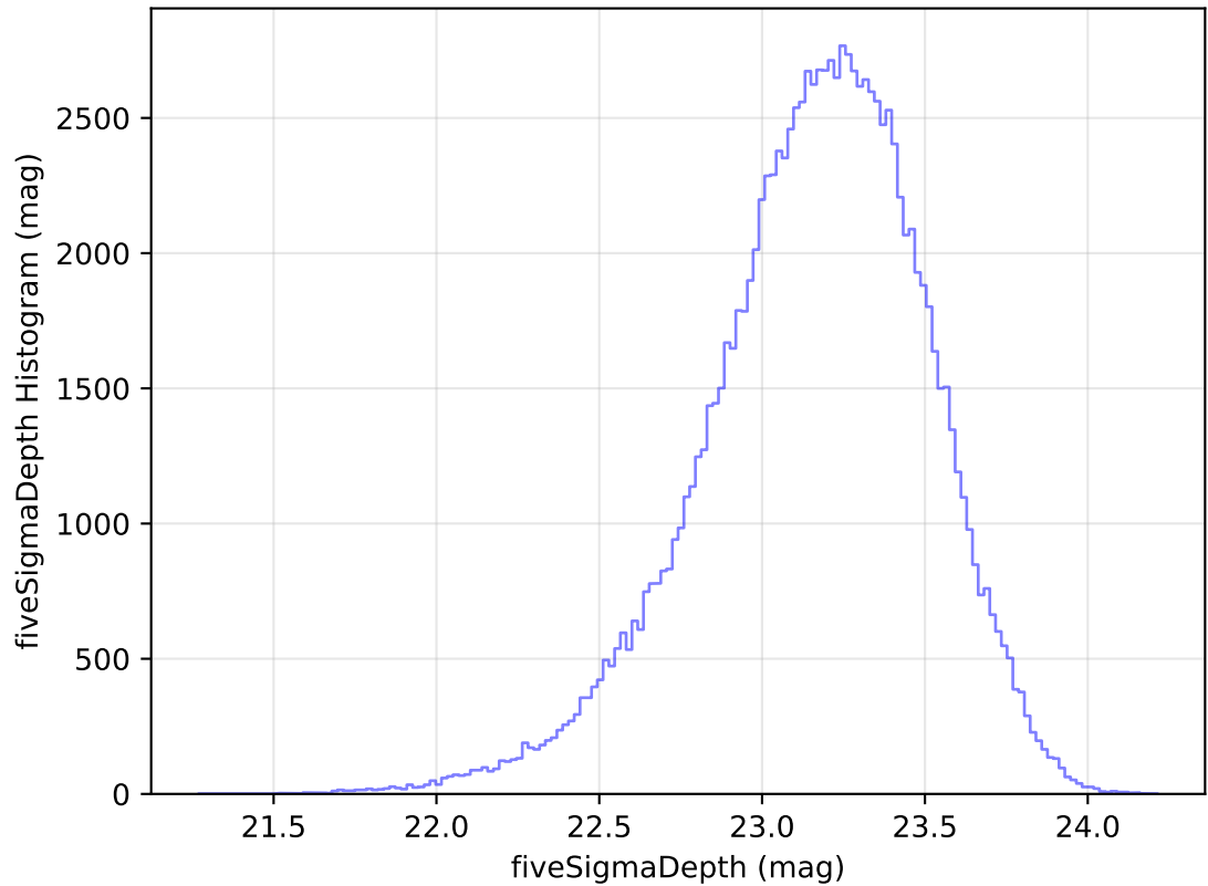
ddf_acor_sf10_lsf30_lsr20_v3.4_10yrs All sky u band: fiveSigmaDepth Histogram
