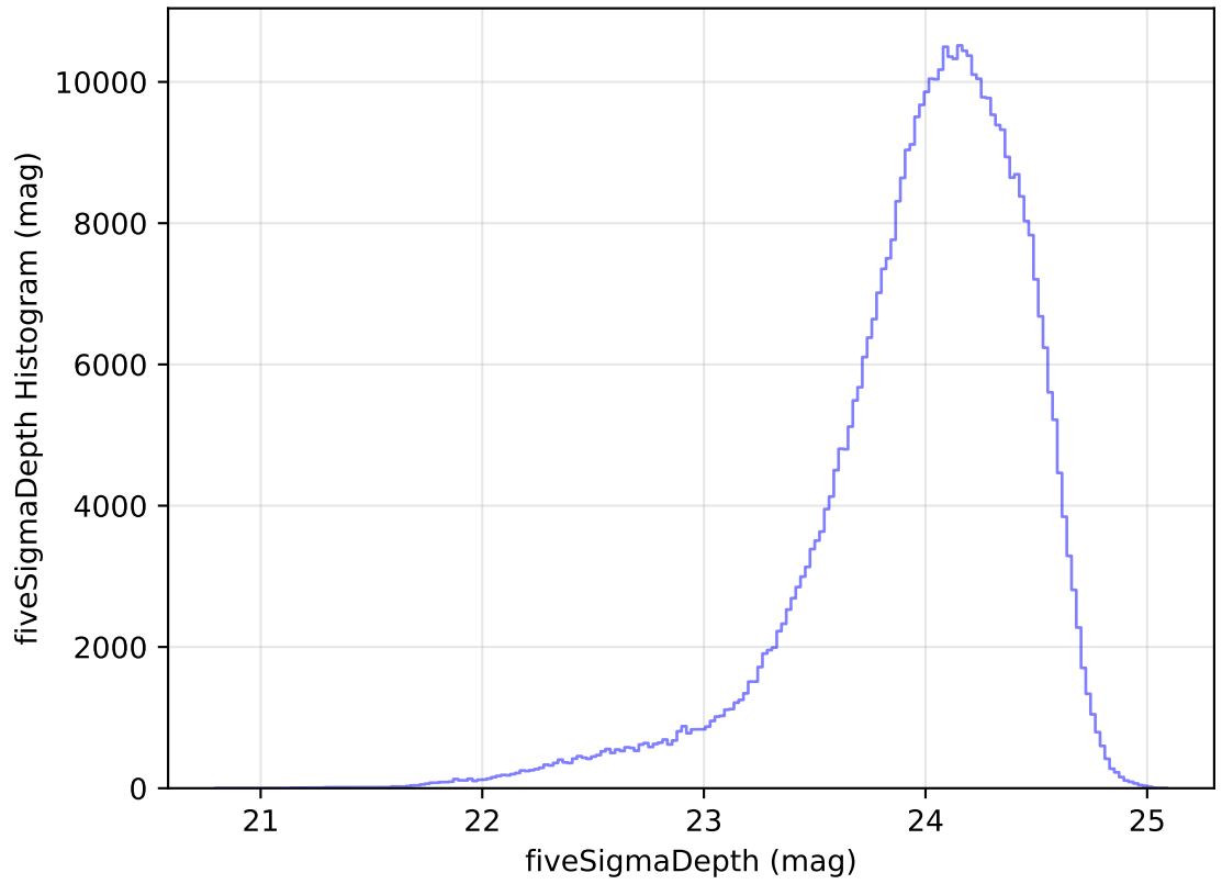
ddf_acor_sf10_lsf30_lsr20_v3.4_10yrs All sky r band: fiveSigmaDepth Histogram
