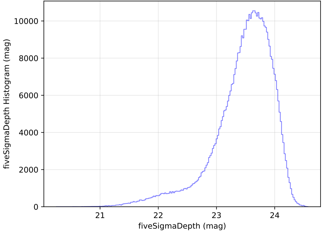
ddf_acor_sf10_lsf30_lsr20_v3.4_10yrs All sky i band: fiveSigmaDepth Histogram
