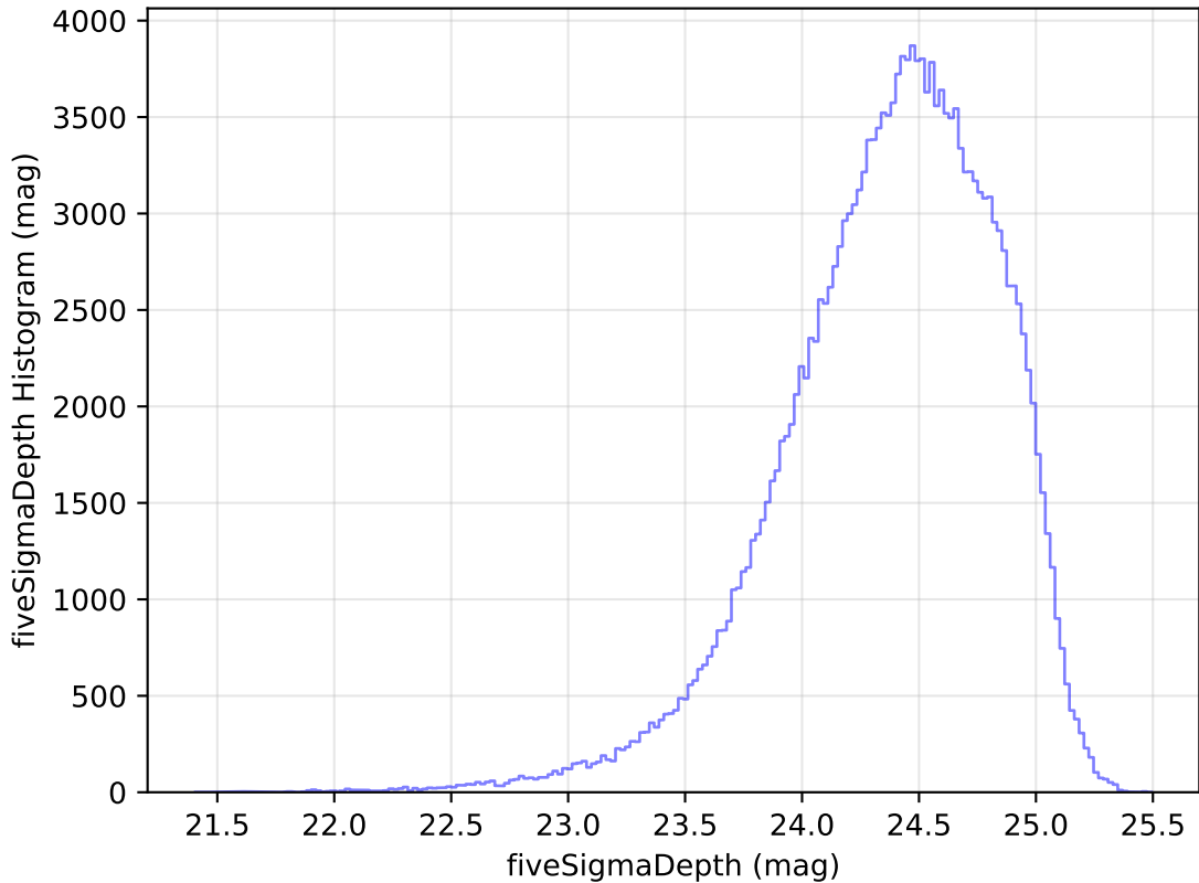
ddf_acor_sf10_ls30_lsr20_v3.4_10yrs All sky g band: fiveSigmaDepth Histogram
