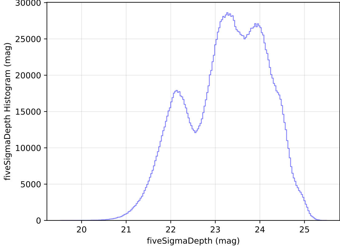
ddf_acor_sf10_lsf30_lsr20_v3.4_10yrs All sky all bands: fiveSigmaDepth Histogram
