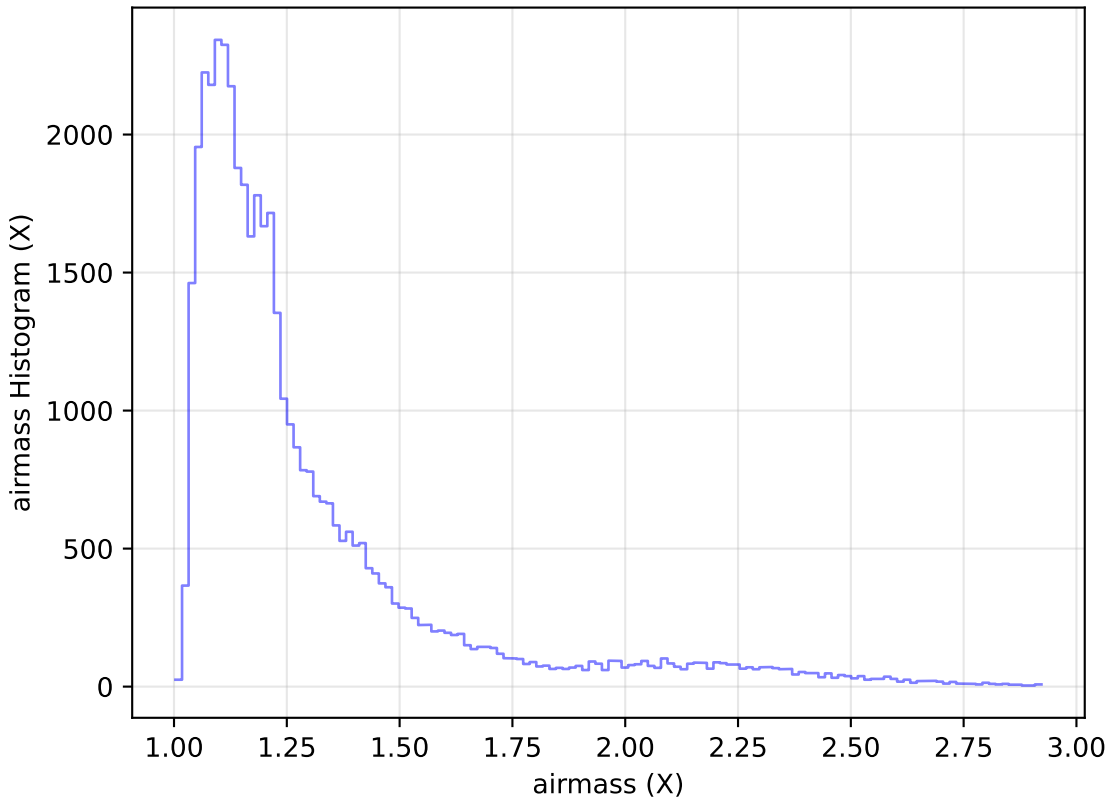
ddf_acor_sf10_lsf30_lsr20_v3.4_10yrs Yr 1 z band: airmass Histogram
