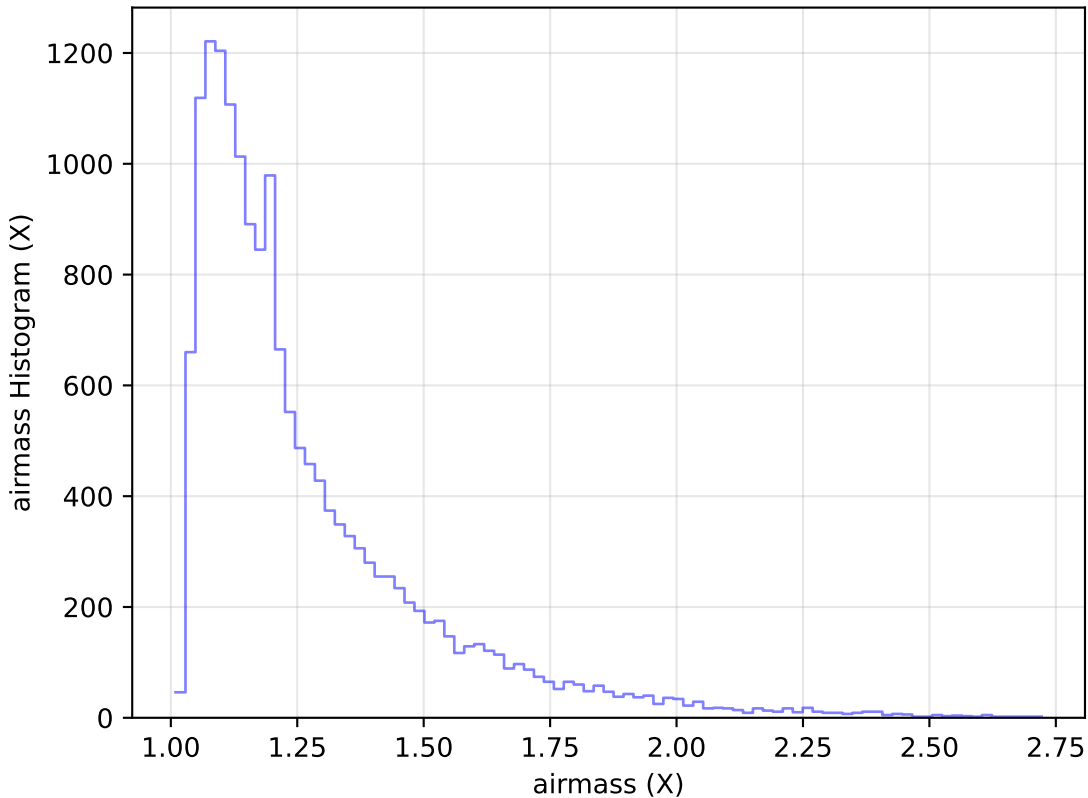
ddf_acor_sf10_lsf30_lsr20_v3.4_10yrs Yr 1 u band: airmass Histogram
