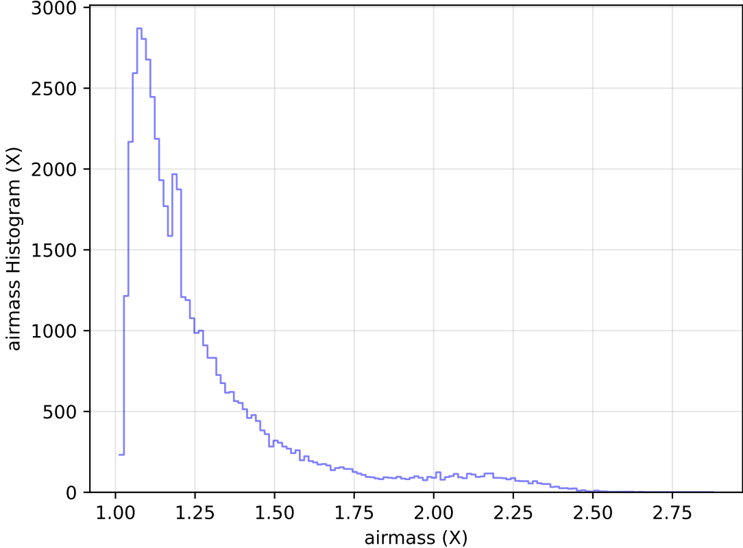
ddf_acor_sf10_lsf30_lsr20_v3.4_10yrs Yr 1 r band: airmass Histogram
