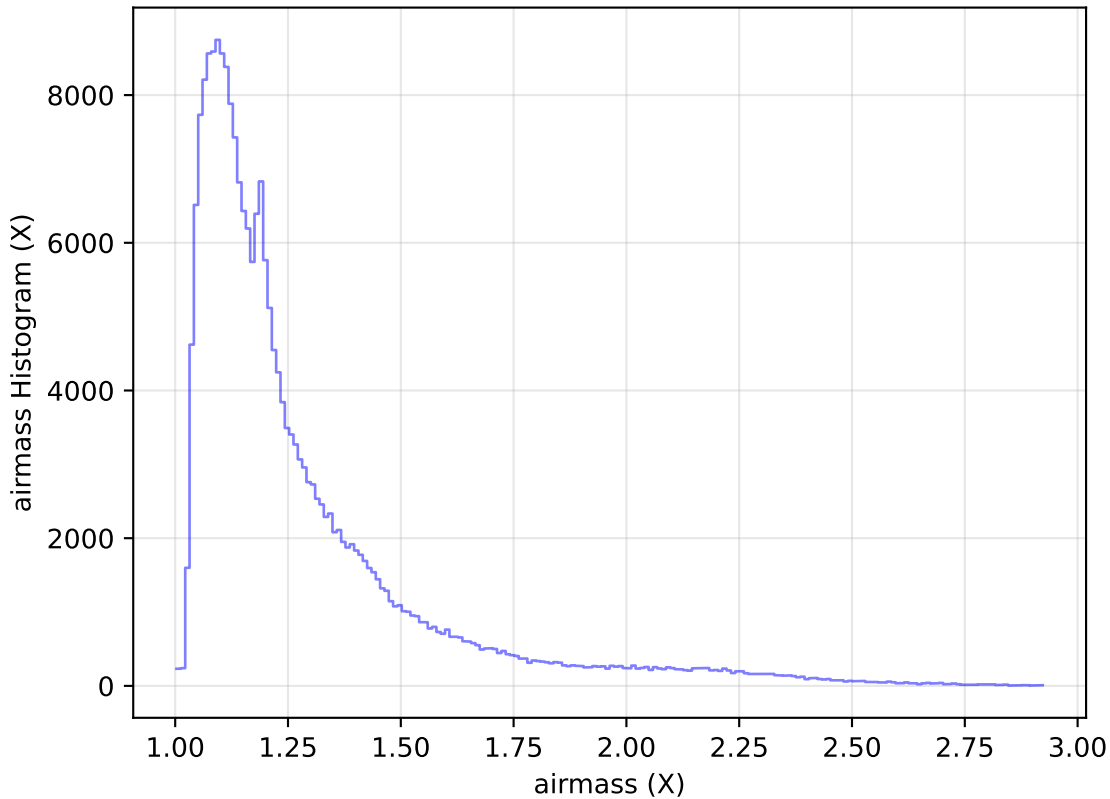
ddf_acor_sf10_lsf30_lsr20_v3.4_10yrs Yr 1 all bands: airmass Histogram
