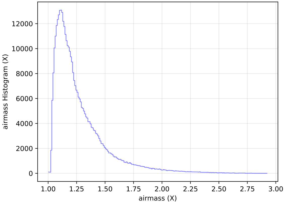
ddf_acor_sf10_lsf30_lsr20_v3.4_10yrs WFD y band: airmass Histogram
